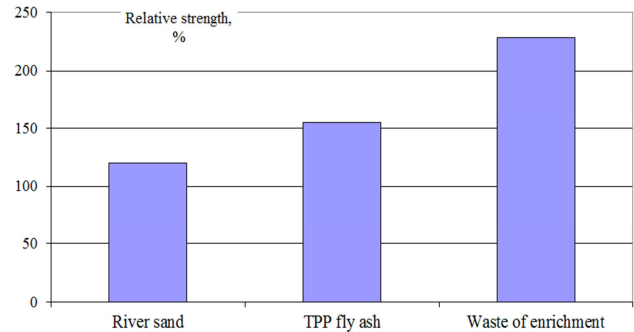
Figure 8. Effectiveness of the application of a reactive powder in the presence of MSAS.
