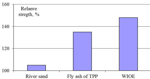
Figure 7. Effectiveness of the application of a reactive powder (without MSAS, WIOE – waste of iron ore enrichment).
