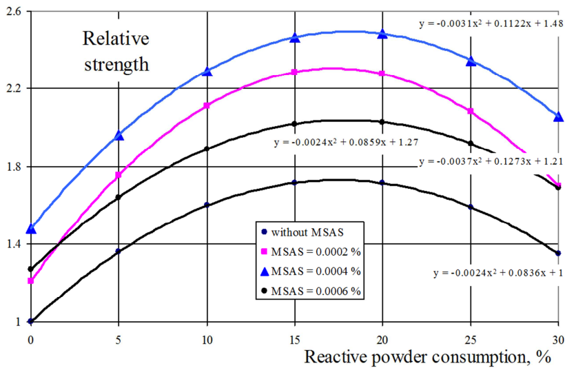
Figure 6. Effect of MSAS content and reactive powder on the strength at compression of the alkaline reactive concrete (reactive powder is the waste of iron ore enrichment).
