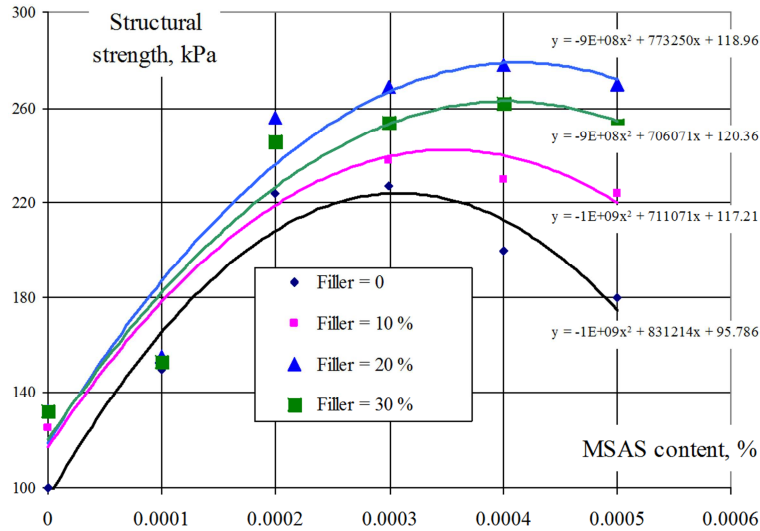
Figure 1. Structural strength of the dispersed system Blast furnace granulated slag – reaction powder – micelle-forming surface-active substance (MSAS) – alkaline component solution: time – 1.2 hours after obtaining the system.
