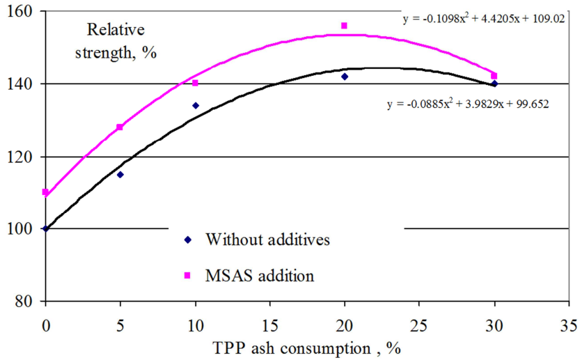
Figure 4. Strength of alkaline reactive concrete.
