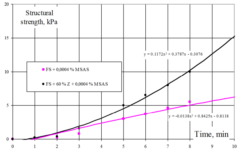
Figure 2. Structural strength of the dispersed system Portland cement – complex SAS (FS – blast furnace granulated slag, Z – reactive powder).
