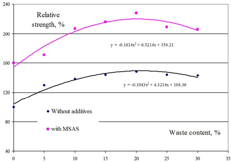
Figure 5. Strength of alkaline reactive concrete.
