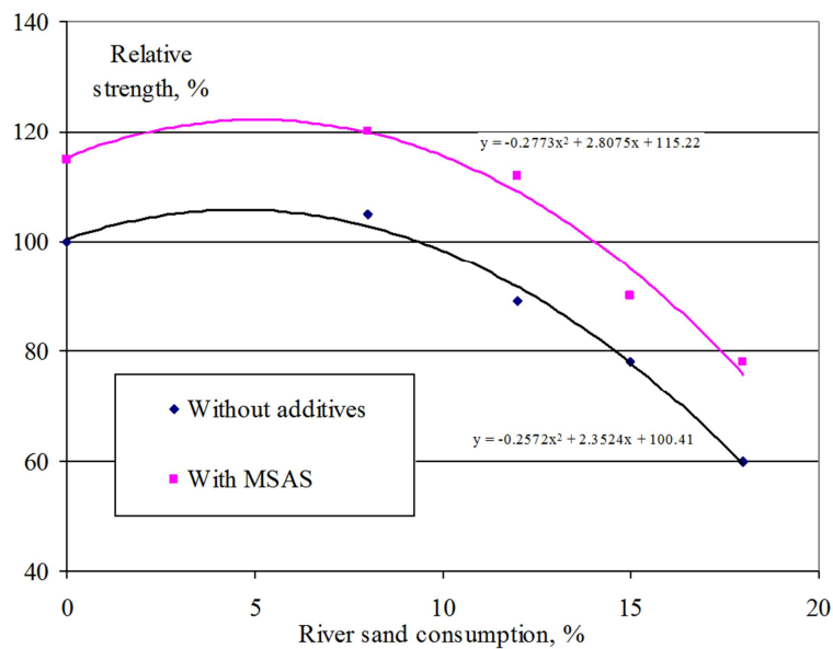
Figure 3. Strength of alkaline reactive concrete.
