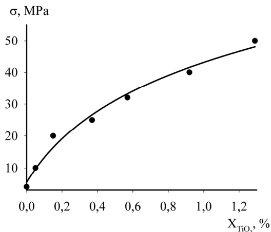
Fig. 9. Dependence of the internal stresses in composites on the content of \text{TiO}_2 in the \text{Cu-TiO}_2 coatings obtained at i=2 \text{ A/dm}^2
