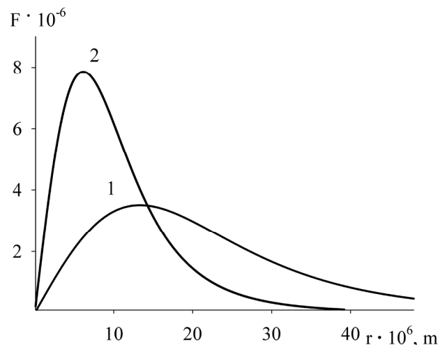
Fig. 10. Differential curves of the \text{TiO}_2 particle distribution by size obtained in methane-sulfonate copper electrolyte containing 2 g/l of titanium dioxide: 1 – without pre-agitation; 2 – with a pre-agitation of the electrolyte for 30 minutes
