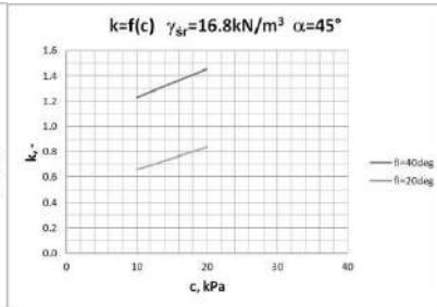
Fig. 3. Cohesion c for (\varphi_{rz}) equal to 40^\circ and 20^\circ and for \varphi_{rz} equal to 45^\circ
