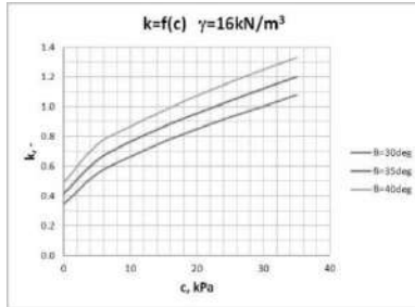
Fig. 2. Cohesion c for different (\varphi_{rz}) and \varphi_{rz} equal to 60^\circ ; k ( F ) - safety factor
